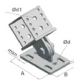
PMKS-MFS-150
